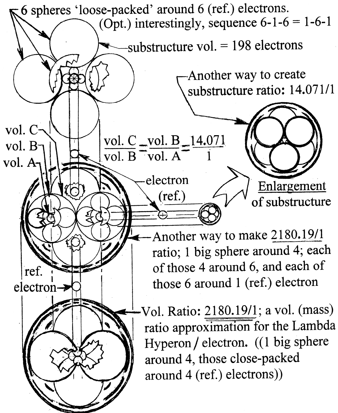
Fig. 2H; the Lambda Hyperon with mass of \frac{2183.34}{1} electrons. Ways to approximate it and its sub-structures.
