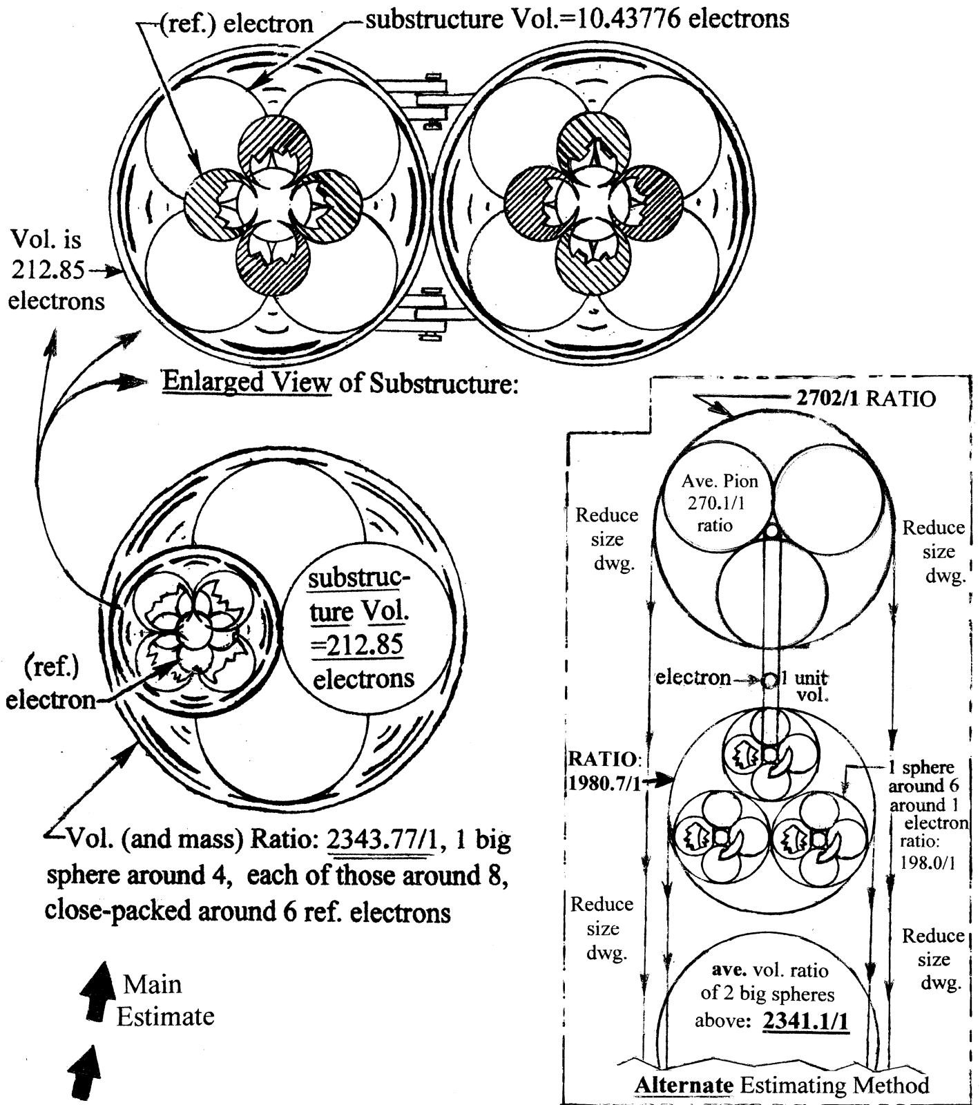
Fig. 4H; Heaviest and longest-life Sigma Hyperon --- empirically equal to 2343.35 electron masses.
