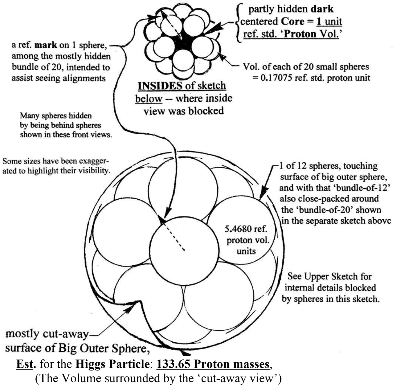
Fig. 12; the Higgs Particle, the above estimate, 133.65 proton masses , is close to (and within experimental errors of) tests thus far performed, giving empirical equivalents of 133.54 proton masses and 134.3 proton masses. Note: Interchanging the '20-spheres' (Dodecahedron) position and the '12-spheres' (Icosahedron) position would not change the Vol. of the outer sphere. (See pg. 13 for an analogy).
